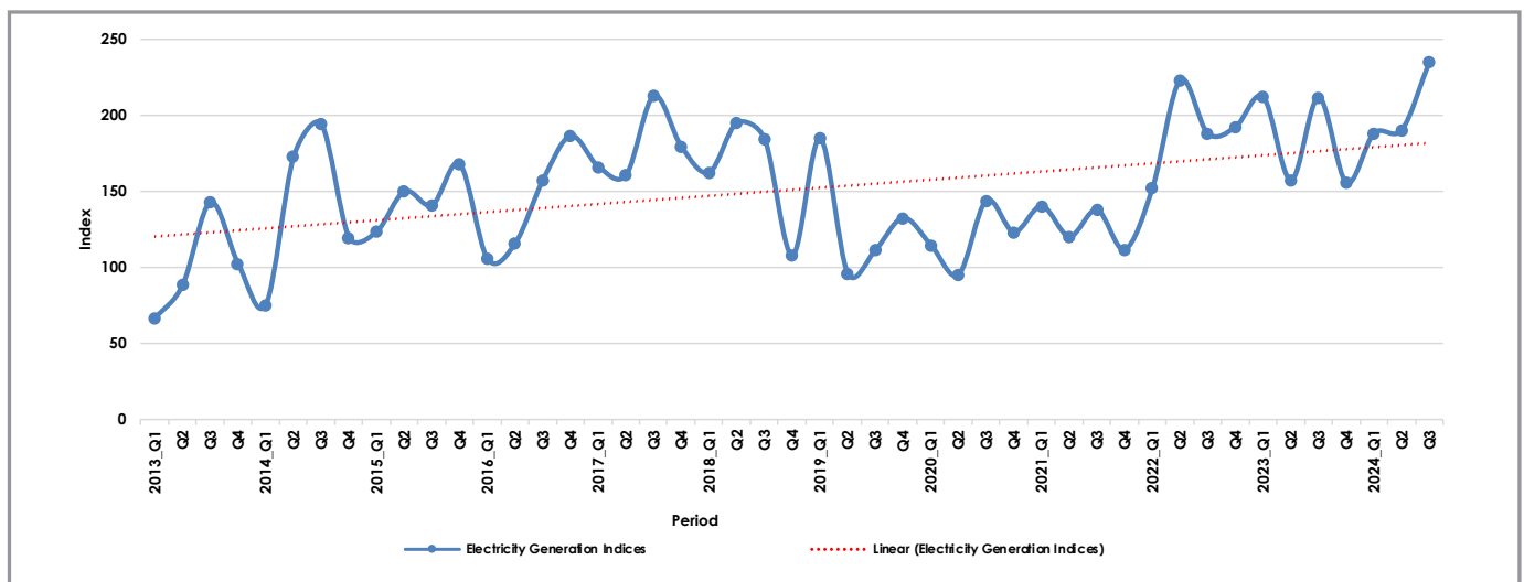
Figure 1: Index of Electricity Generation (MWH): 2013 First Quarter to 2024 Third Quarter
